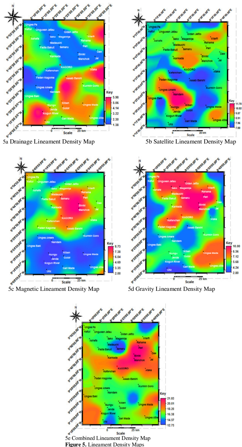
Figure 5. Lineament Density Maps
