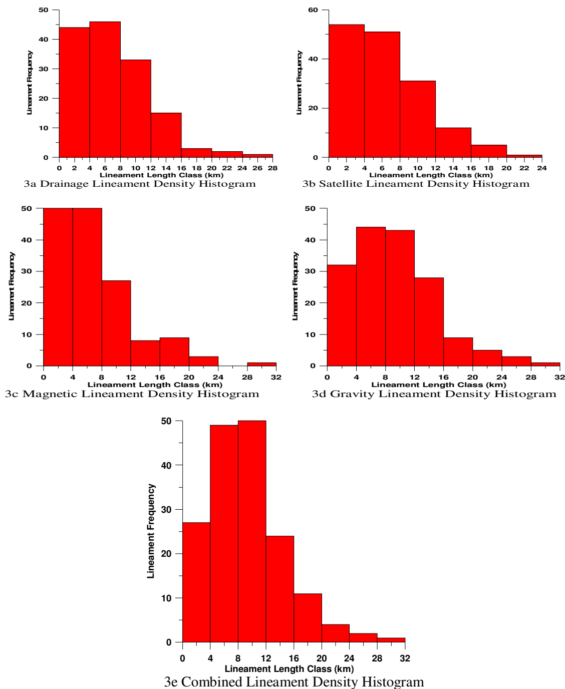
Figure 3. Lineament Density Histograms
