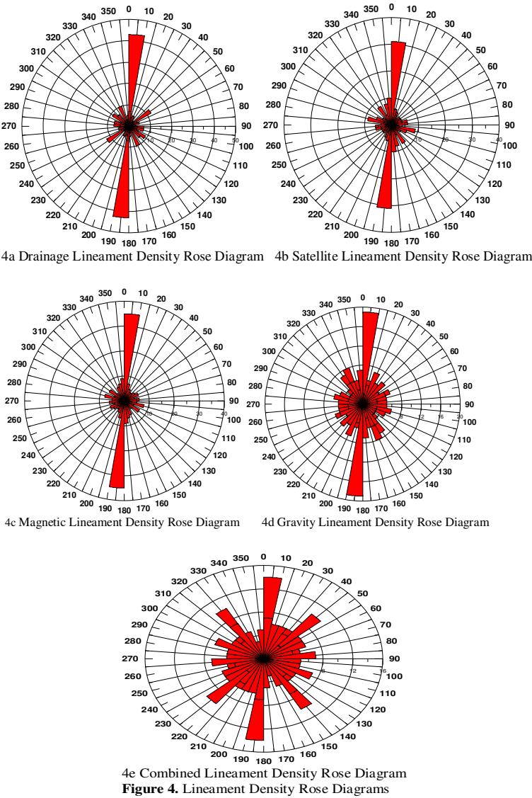
Figure 4. Lineament Density Rose Diagrams
