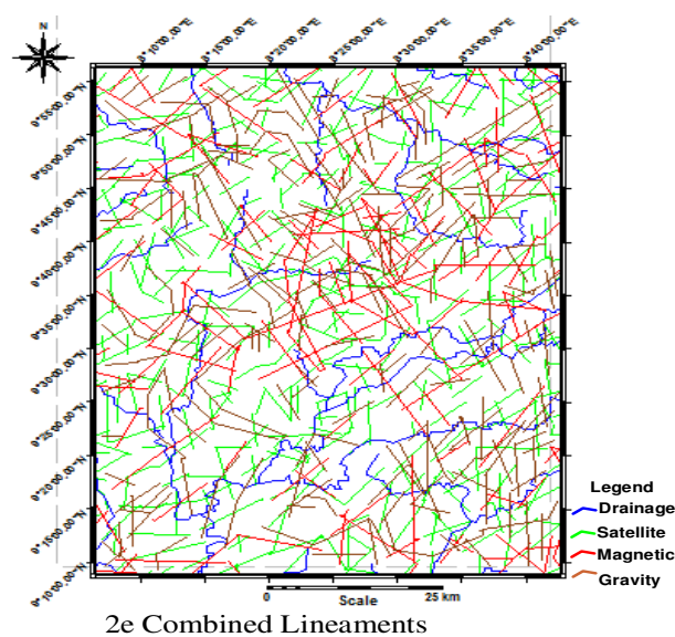
Figure 2. Source Data of the Lineaments
